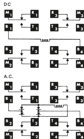
Wiring Diagrams (Bottom Views)
