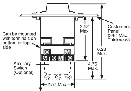
Panel Mount Option "X"
