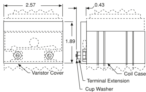
Surge/Transient Protection Option
